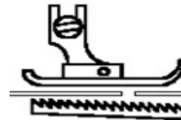
(c) Position of the feed dog with its side opposite the operator in a raised position.
