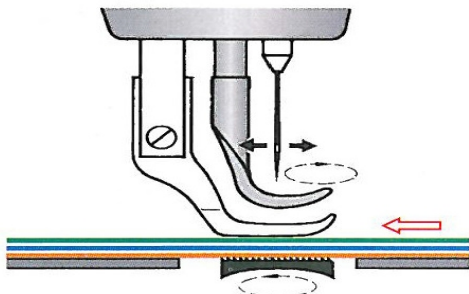
Figure (4): Unison feed mechanism
