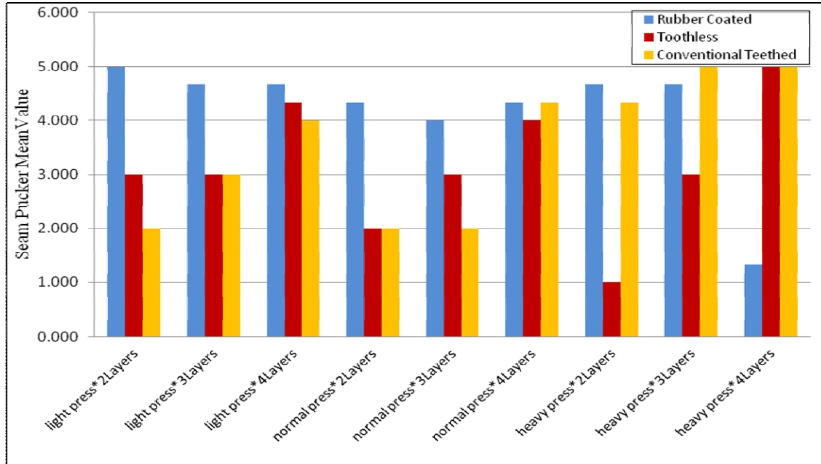
Figure (13): Effect of using modified feed-dogs on mean values of seam pucker test
