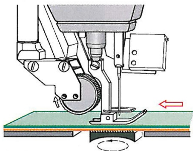
Figure (5): Puller feed mechanism
