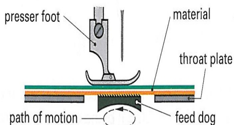
Figure (1): Drop feed mechanism
