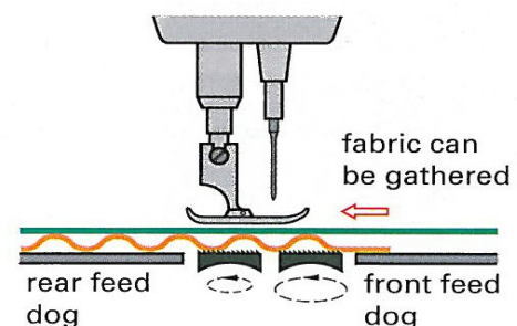
Figure (2): Differential feed mechanism
