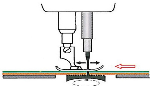
Figure (3): Compound Needle feed mechanism
