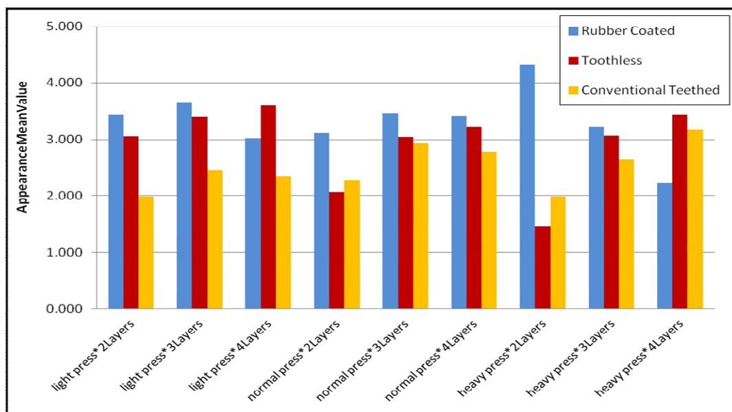
Figure (12): Effect of using modified feed-dogs on mean values of appearance test
